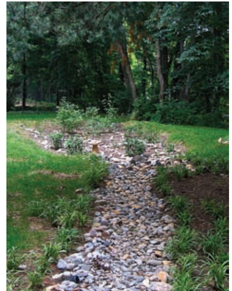
A stone-lined swale serves as the inlet structure for a rain garden in Merrifield.
